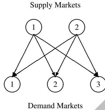
Figure 3: The Network Structure of the Spatial Price Equilibrium Example 3.4, 3.5, and 3.6 Problems
